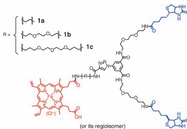
Scheme 1. Molecular structures of the heme-bis(biotin) dyads 1a–c .
