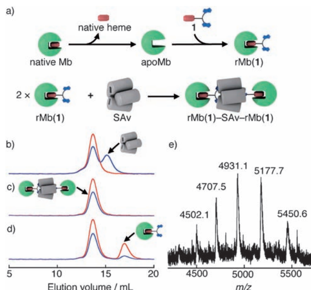
Figure 1. Assembly of rMb(1b) and SAv. a) Schematic representation of reconstitution of Mb with 1 and formation of rMb(1b)-SAv-rMb(1b). SEC traces of complexation of SAv with b) one, c) two, and d) three equivalents of rMb(1b) compared to SAv. The red and blue traces show the absorbance at 408 and 280 nm, respectively. e) ESI-TOF MS spectrum of rMb(1b)-SAv-rMb(1b); calculated m/z ( z ) = 5450.4 (19+), 5177.9 (20+), 4931.4 (21+), 4707.3 (22+), and 4502.7 (23+).
